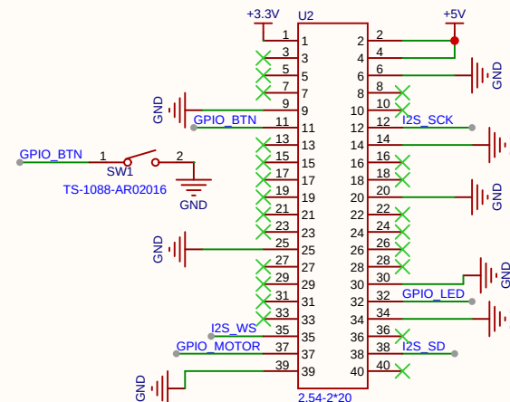
SBC 40-pin
